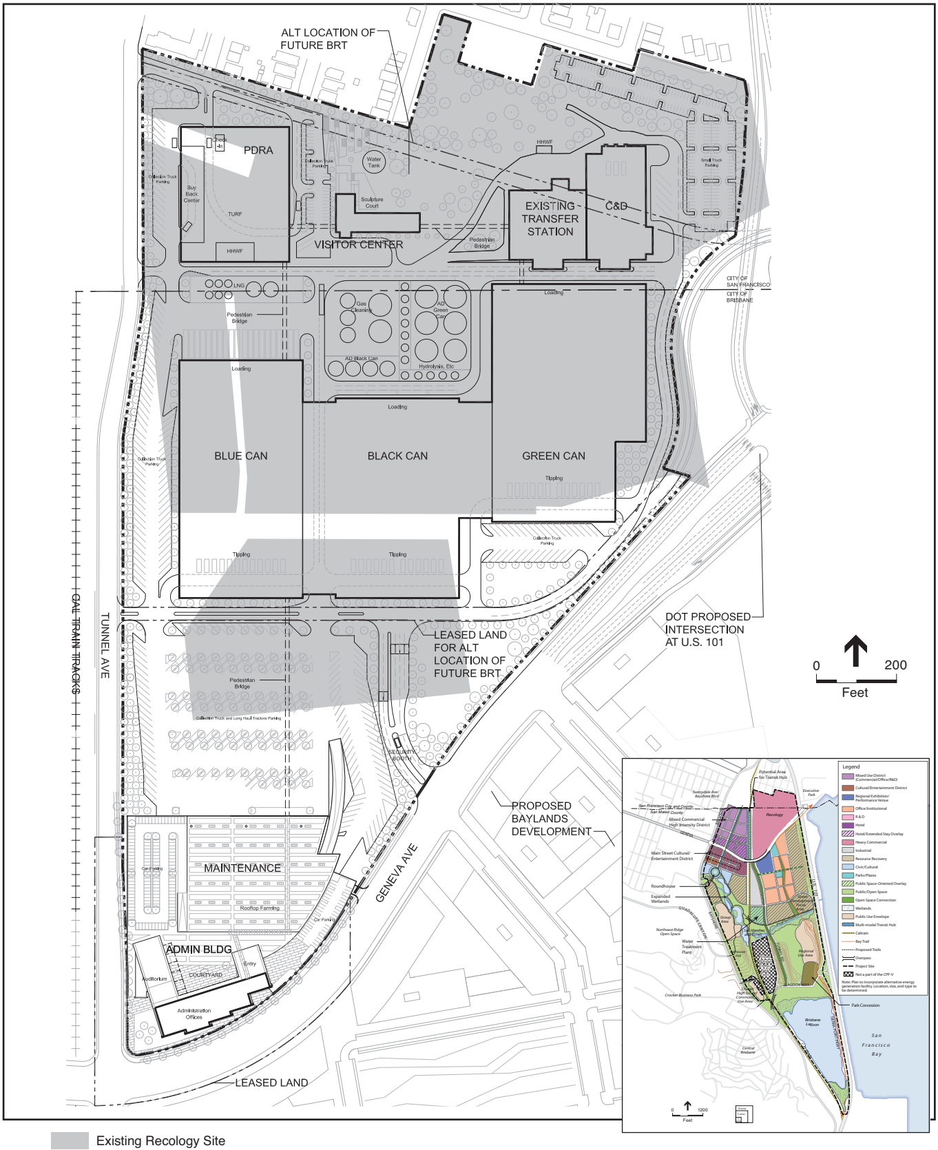
Figure 8 Community Proposed Plan (CPP) Recology Expansion Variant Proposed Site Plan
