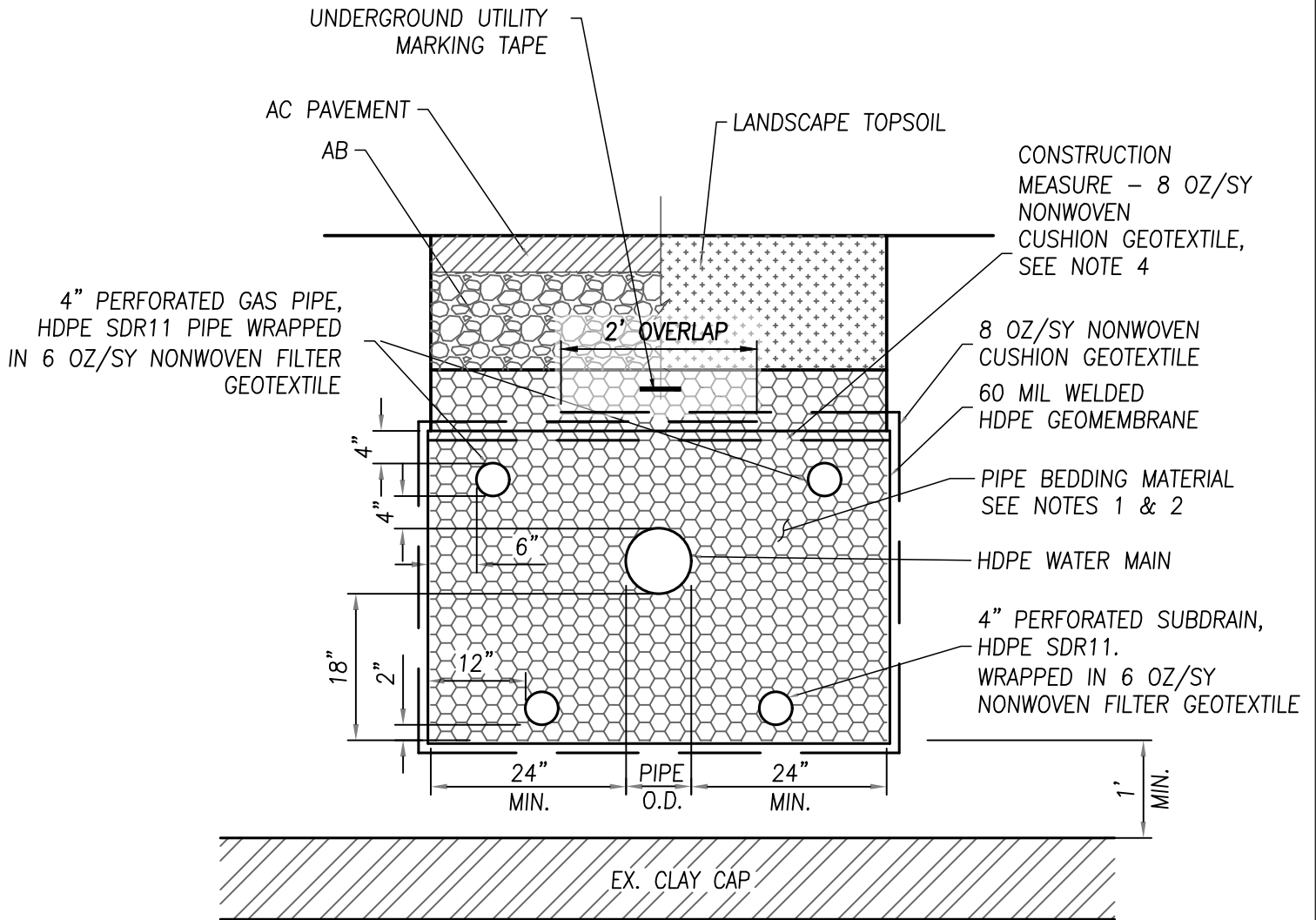
TYPICAL SECTION
